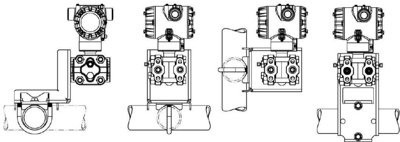
Figure 4 – Mounting Configurations
